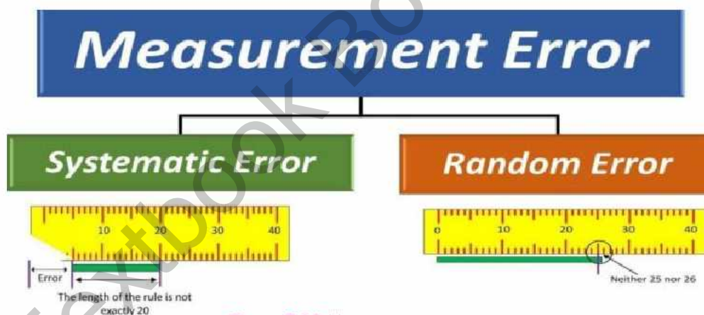
Figure 7.10 Measurement errors
