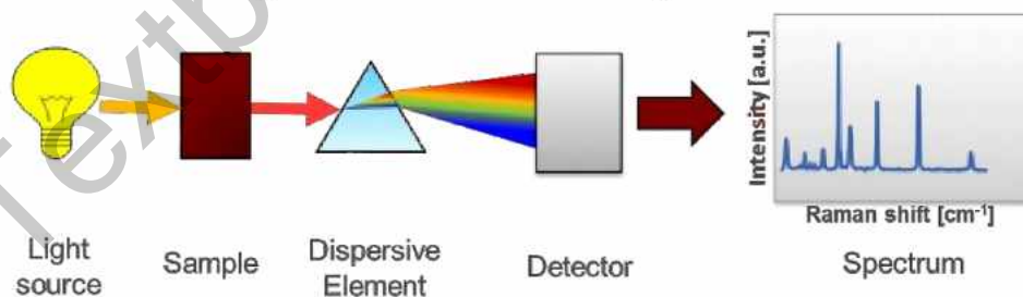
Figure 7.13 Spectroscopic methods
