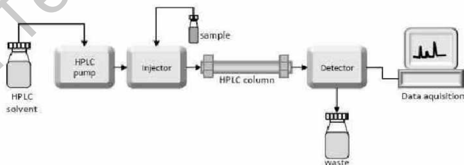
Figure 7.17 HPLC
