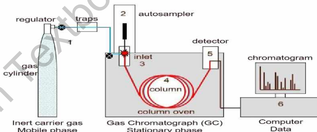
Figure 7.18 Gas chromatography
