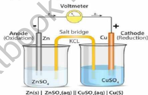
Figure 7.19 Electrochemical cell
