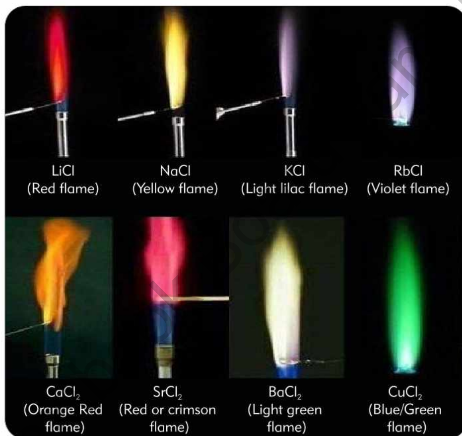
Figure 7.2 Flame test
