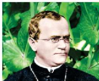
FIGURE 7.5: Gregor Mendel
