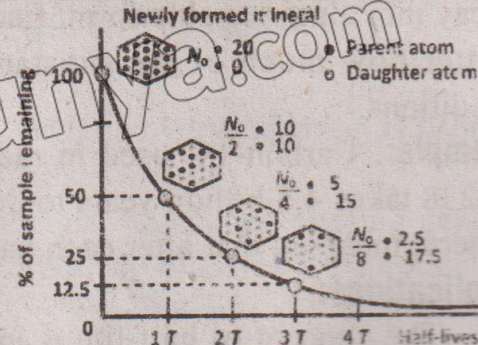
Fig. 20.14: Conversion of ^{99}\text{Tc} to ^{99}\text{Ru} by beta decay
