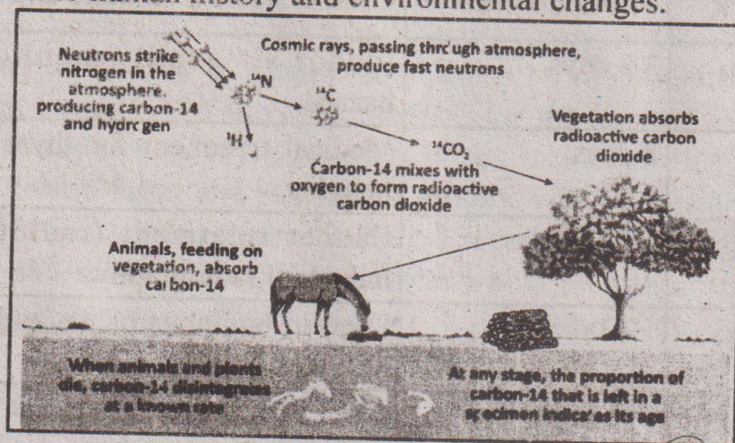
Fig. 20.15: Carbon dating
