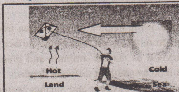
Fig. 11.4: Sea breeze blows from sea to land as warm air rises over heated land (day time)
