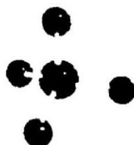
Structure of Methane (CH 4 )
