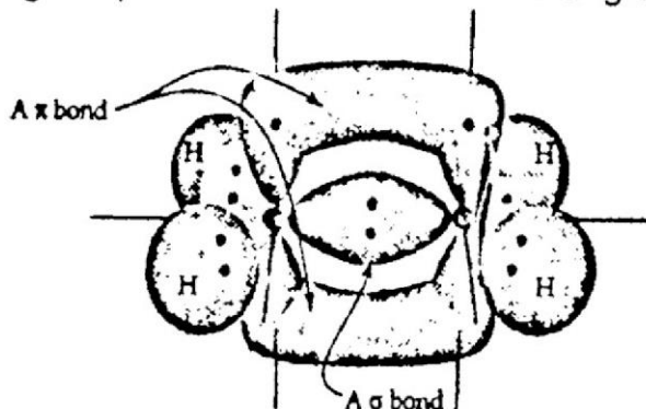
Structure of Ethene ( CH_2 = CH_2 )
