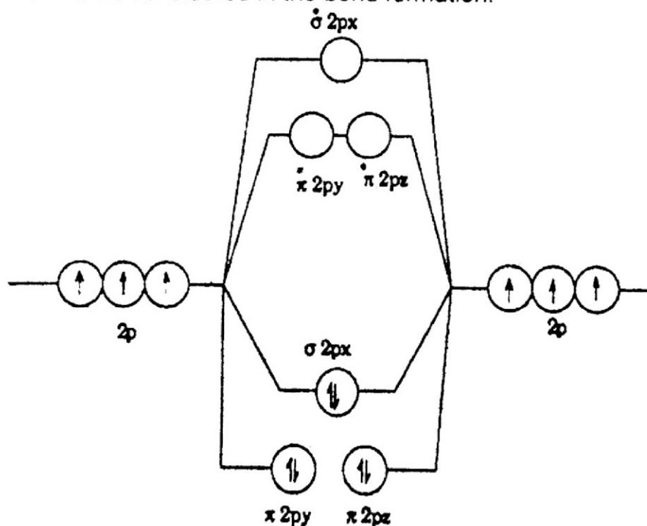
Molecular orbitals energy level diagram of N 2
