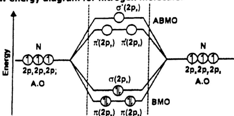
Molecular orbitals energy level diagram of N_2
