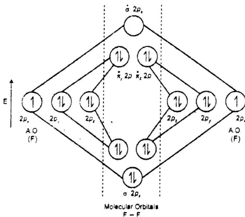
Molecular orbitals energy level diagram of F_2
