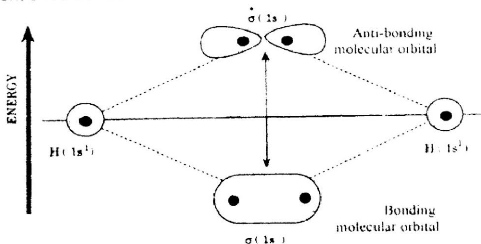
Energy diagram of bonding and anti-bonding molecular orbitals
