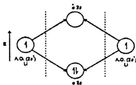
Molecular orbitals energy level diagram of \text{Li}_2
