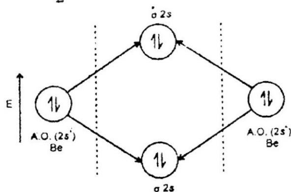
Molecular orbitals energy level diagram of \text{Be}_2
