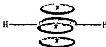
formation of \pi bonds
