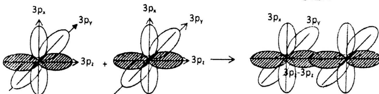
Orbital diagram of \text{Cl}_2
