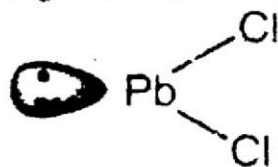
V. shaped \text{PbCl}_2 molecule
