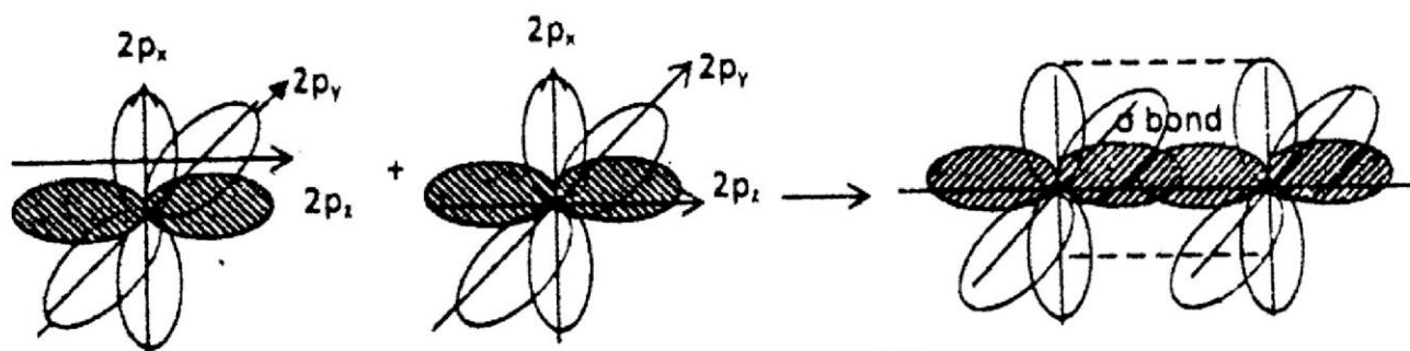
Orbital diagram of F_2
