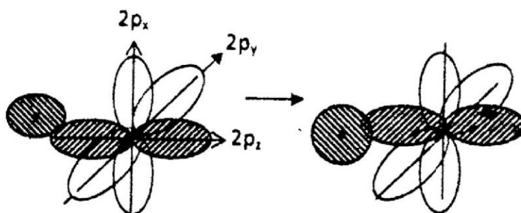
Orbital diagram of HF
