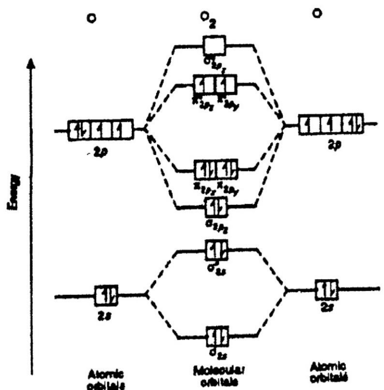
Molecular orbitals energy level diagram of \text{O}_2
