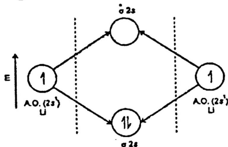
Molecular orbitals energy level diagram of \text{Li}_2
