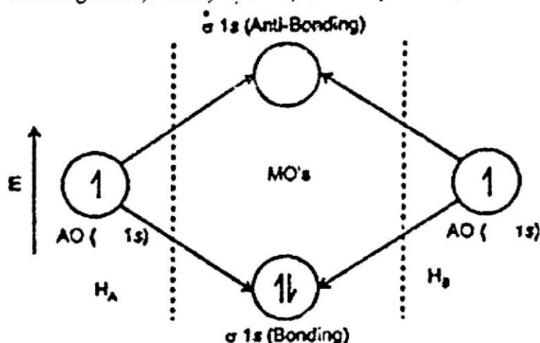
Molecular orbitals energy level diagram of \text{H}_2
