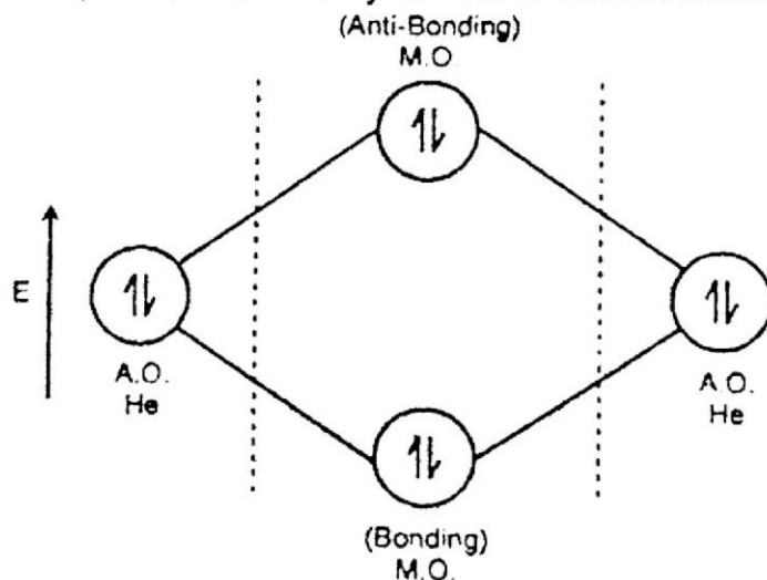
Molecular orbitals energy level diagram of \text{He}_2
