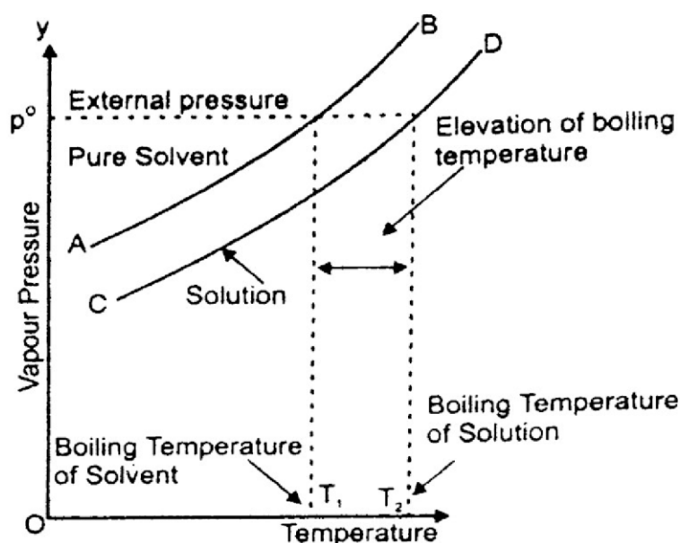
Elevation of boiling point - temperature curve
