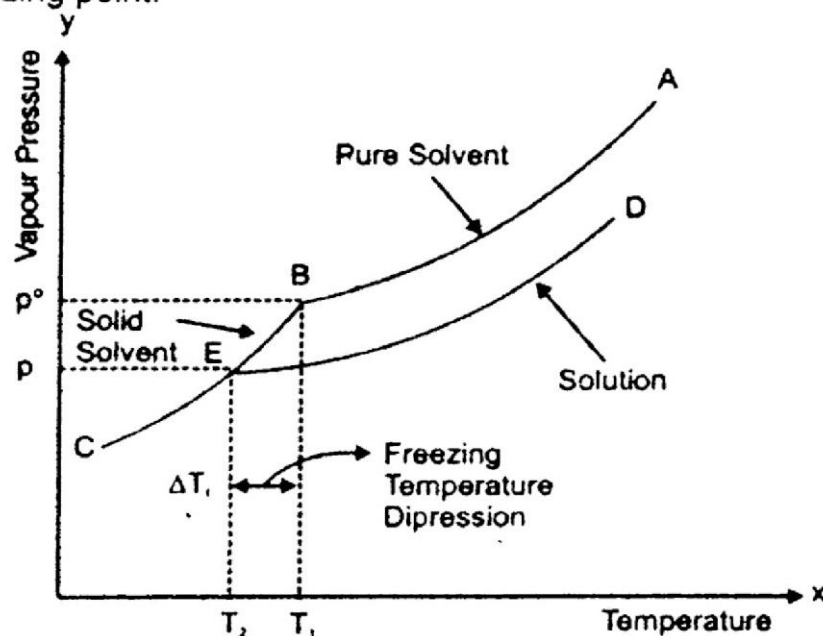
Depression of freezing point – temperature curve
