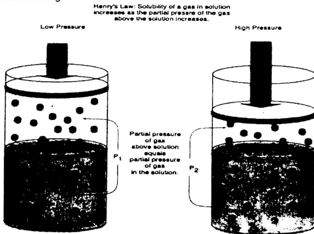
Schematic representation of Henry's law
