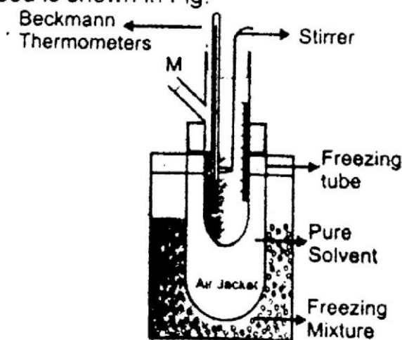
Beckmann's apparatus for measurement of depression of freezing point.
