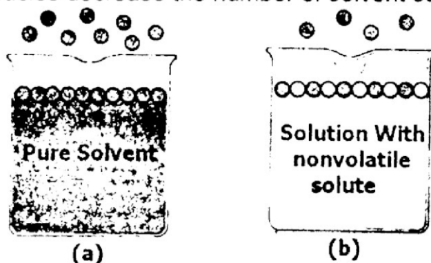
Lowering of vapour pressure
