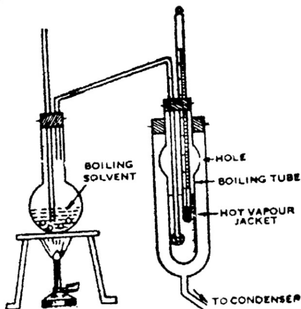
Landsberger's apparatus for measurement of elevation of boiling points.
