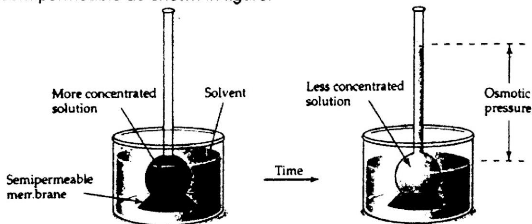
The phenomenon of osmosis
