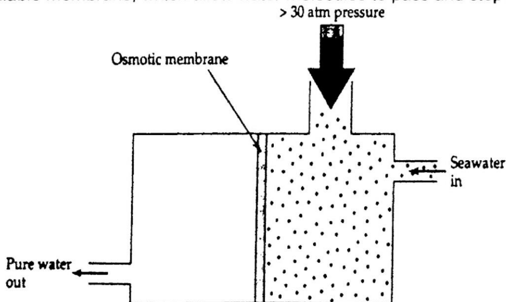
A schematic for the desalination of seawater by reverse osmosis
