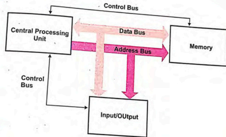
Figure 3.4 System Buses
