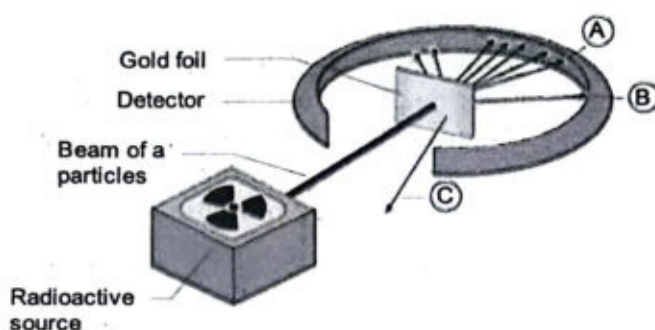
Fig. 4.4: Rutherford's Experiments
