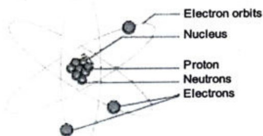
Fig. 4.5: Rutherford Atomic Model
