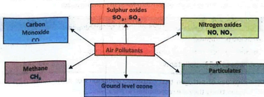
Figure 11.2: Air pollutants
