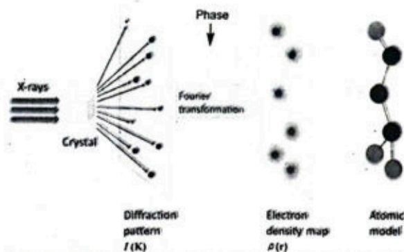
Fig 20.11 X-ray Crystallography
