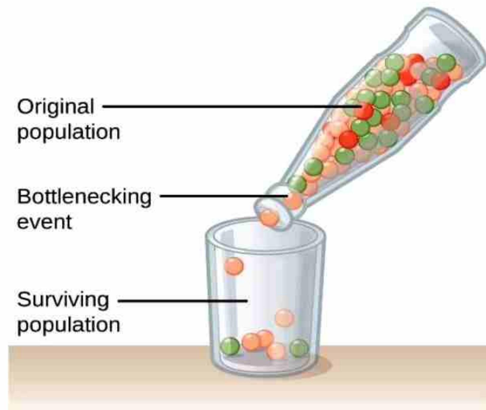
Fig. 24.12 Bottle-neck Effect
