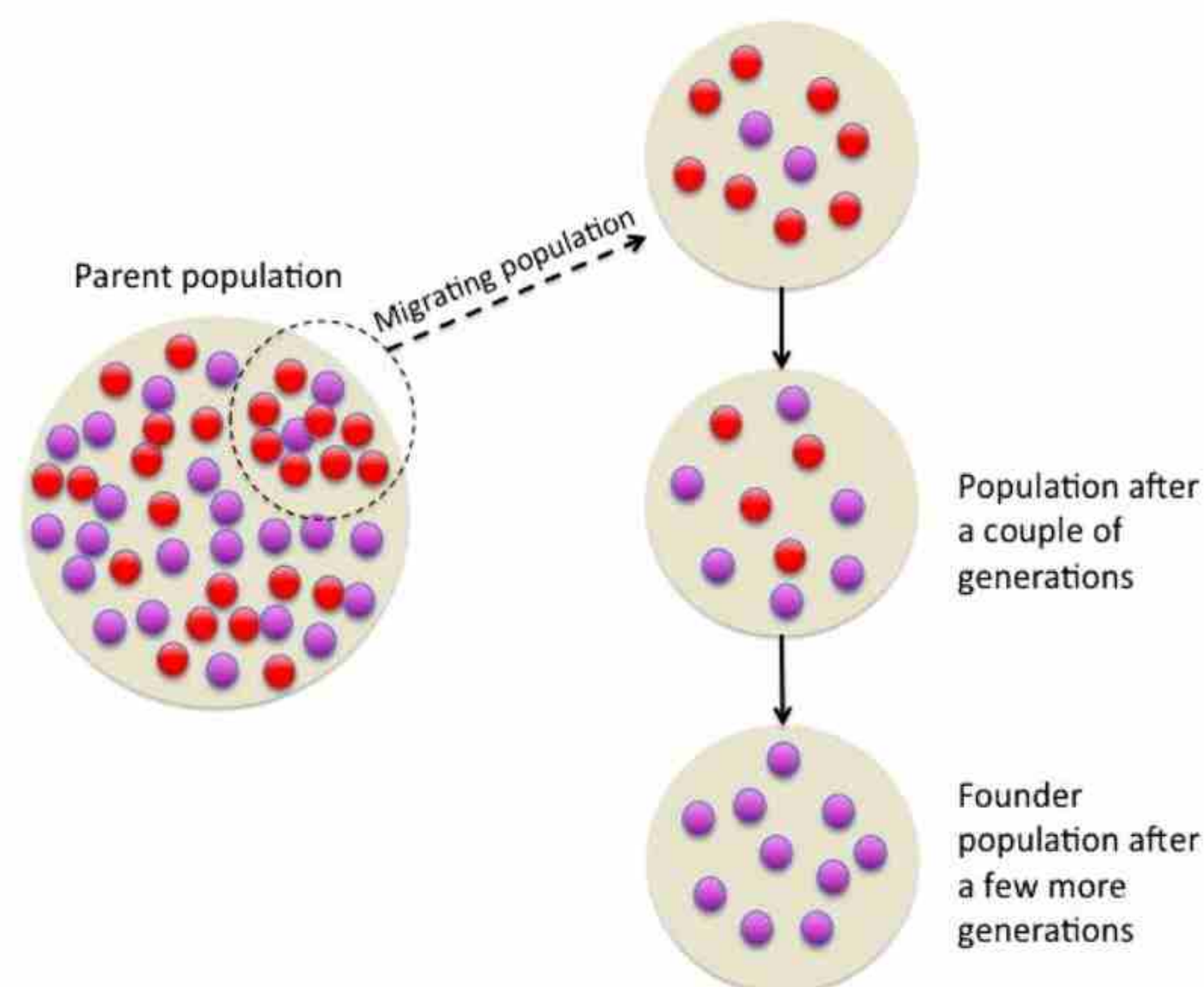
Fig. 24.13 Founder's Effect
