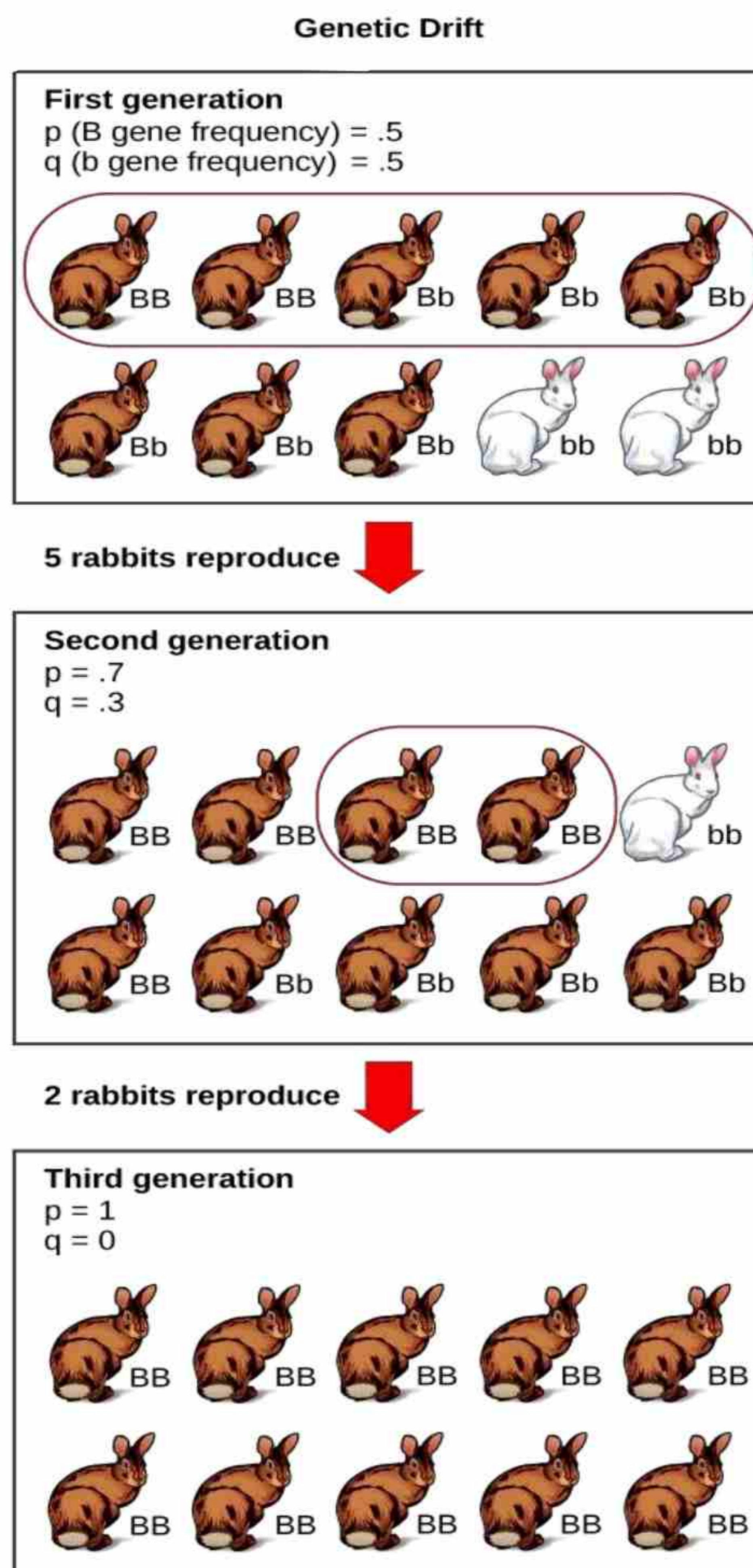
Fig. 24.10 Genetic drift
