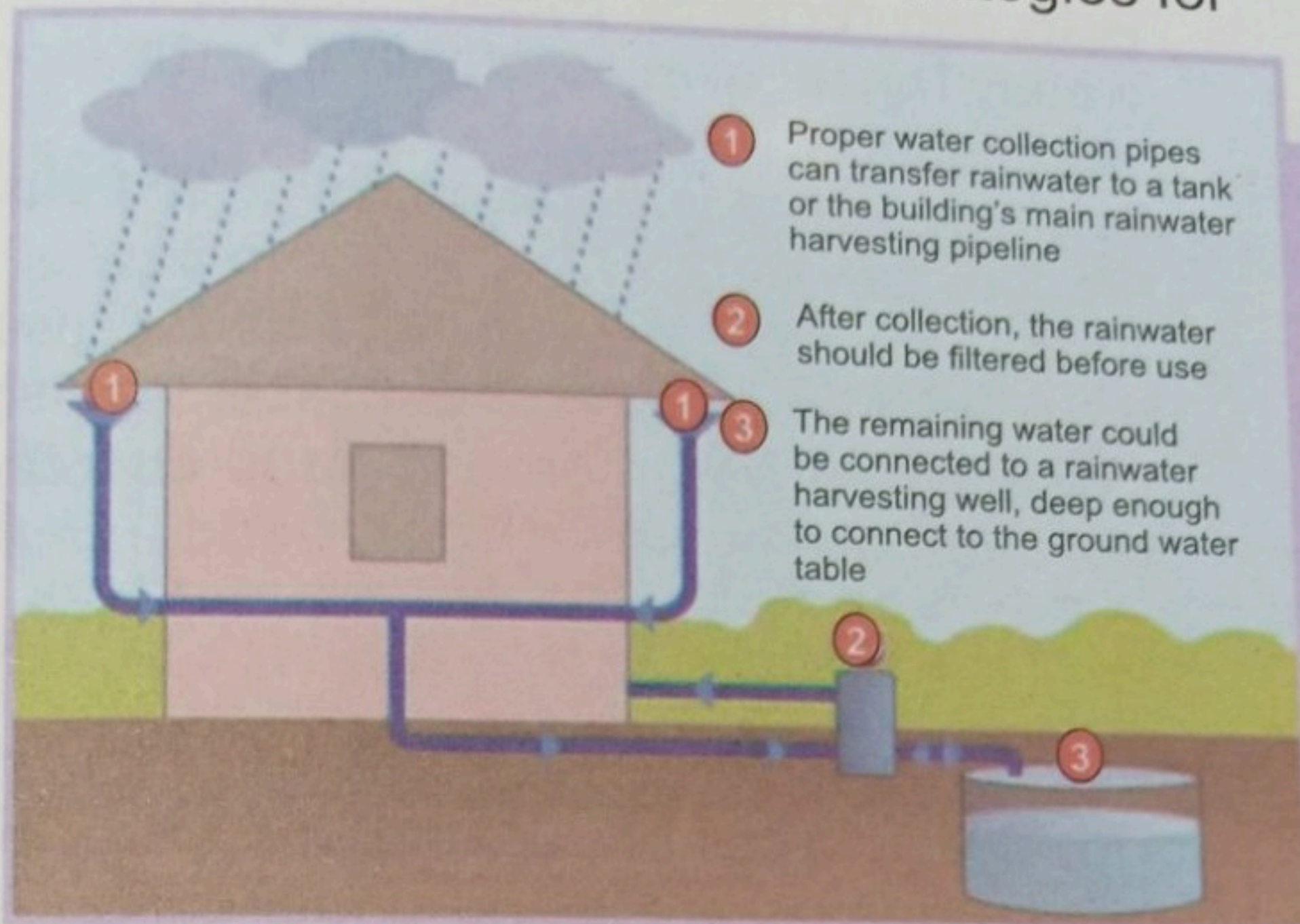
Fig: 9.10 Rain harvesting system
