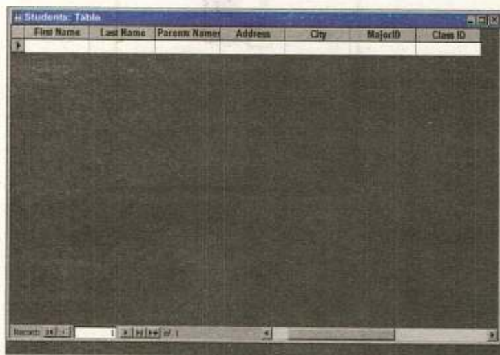
Fig. 6.2 Datasheet View
