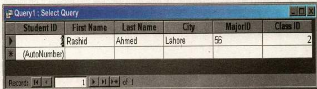
Fig.5.9 Select Query
