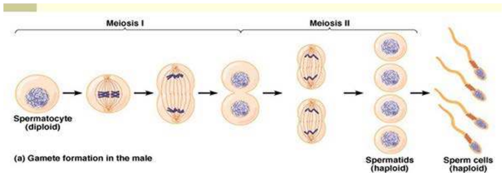
Fig. 18.3 Gamete formation
