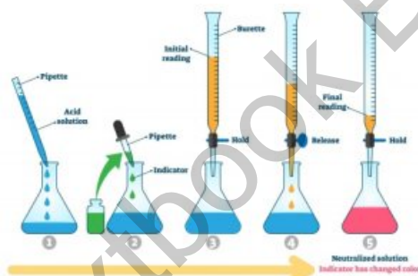
Figure 7.12 Titration
