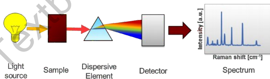
Figure 7.13 Spectroscopic methods
